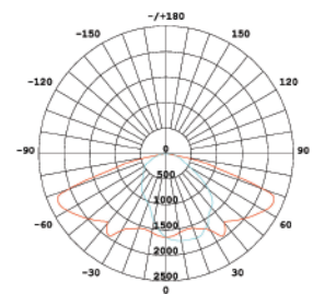
DUAPLM1 Iso-brightness
