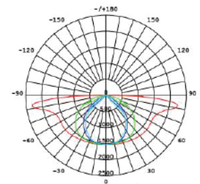
DUAPLM2 Iso-brightness
